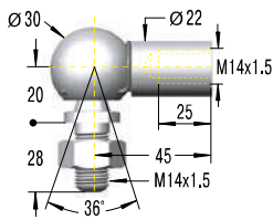
C14-VA Angle Ball Joint
