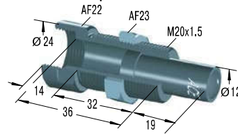
BV20SC Side Load Adaptor
