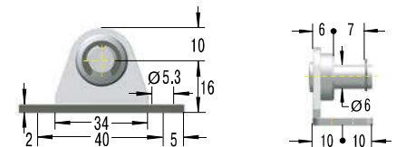
NA5-V4A Angle Bracket with Ball
