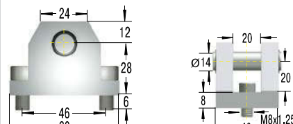
ME14-VA Bearing Shoe
