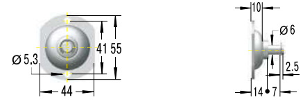
PA5-V4A Round Bracket with Ball
