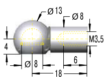
G3,5-V4A Ball Socket
