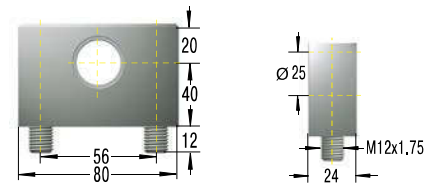
ND24 Mounting Flange
