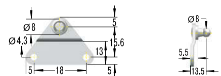
OG3,5-V4A Side Bracket with Ball
