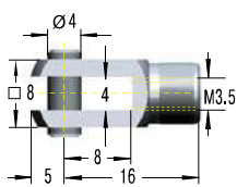
D3,5-V4A Clevis Fork
