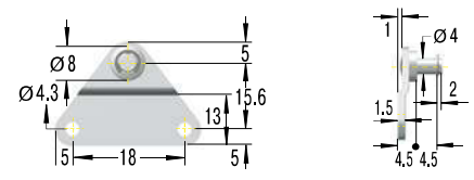
OA3,5-V4A Side Bracket with Ball
