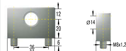
ND14-VA Mounting Flange
