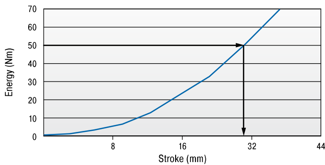
Type TR93-57 Energy-Stroke Characteristic (dynamic) (with impact velocity over 0.5 m/s)
