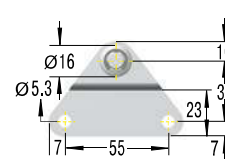
OE10 Side Bracket with Ball
