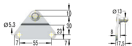
OG8-V4A Side Bracket with Ball
