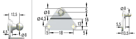
OG3,5 Side Bracket with Ball
