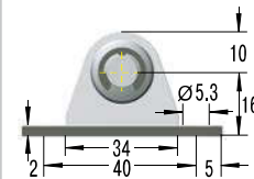
NE8 Angle Bracket with Ball
