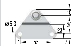
OG8 Side Bracket with Ball
