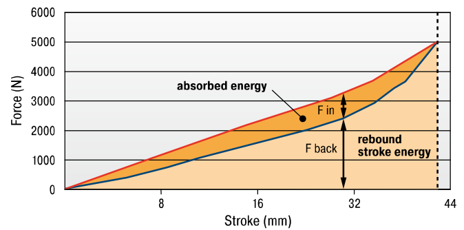
Type TR93-57 Force-Stroke Characteristic (dynamic) (with impact velocity over 0.5 m/s)
