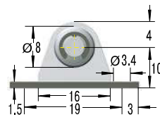
NA3,5-V4A Angle Bracket with Ball
