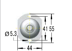
PE8 Round Bracket with Ball
