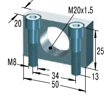
MB20SC2 Mounting Block
