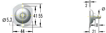
PG5-V4A Round Bracket with Ball
