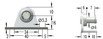
NA5 Angle Bracket with Ball
