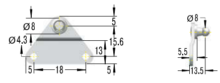
OG5 Side Bracket with Ball
