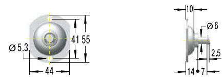
PA5 Round Bracket with Ball
