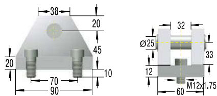
ME24 Bearing Shoe
