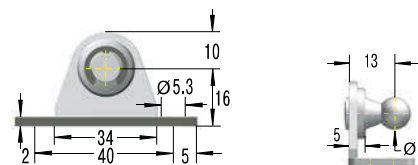
NG5 Angle Bracket with Ball
