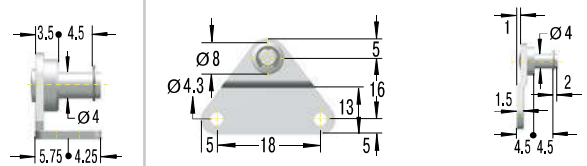
OA3,5 Side Bracket with Ball
