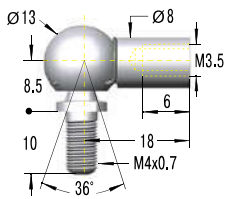
C3,5-V4A Angle Ball Joint
