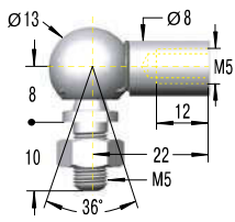
C5-VA Angle Ball Joint
