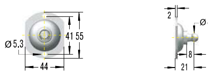
PG5 Round Bracket with Ball
