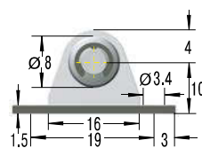
NG3,5-V4A Angle Bracket with Ball
