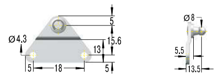
OG5-V4A Side Bracket with Ball
