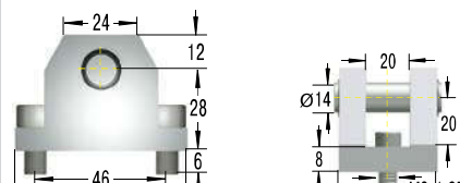
ME14-VA Bearing Shoe
