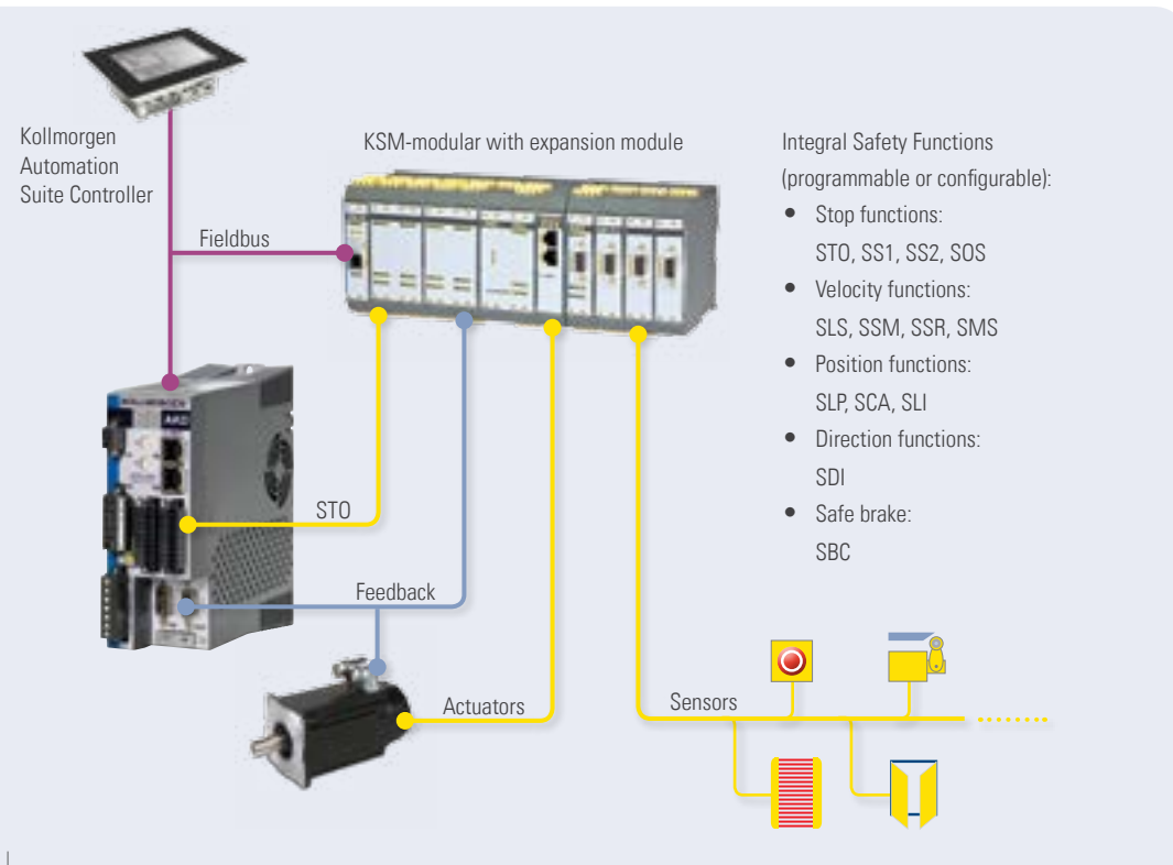
Example solution using the Kollmorgen Motion Safety concept.
