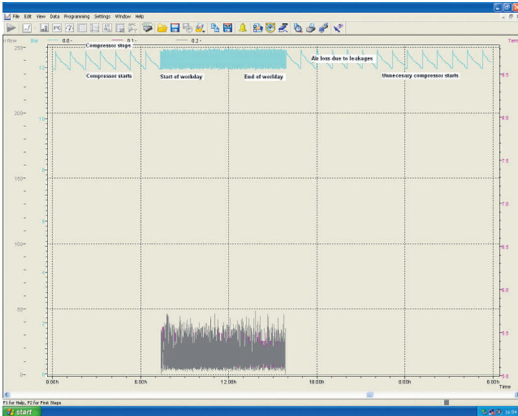
Graph A: compressed air system without an AIR-SAVER
