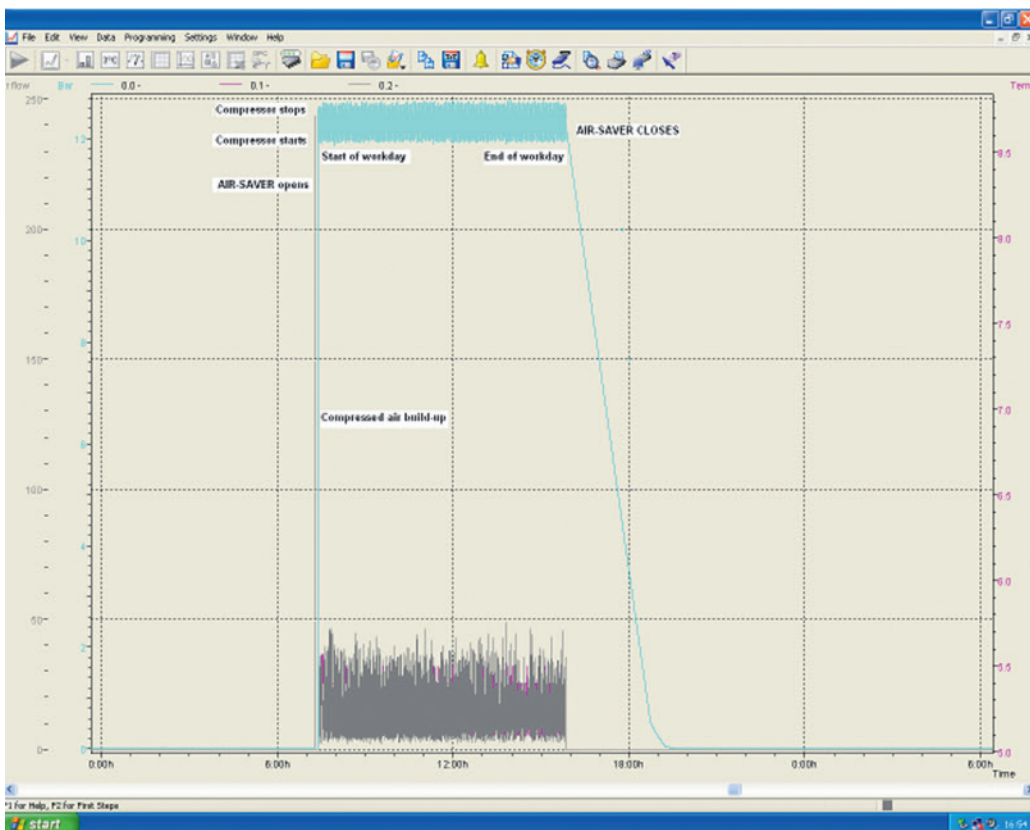
Graph B: compressed air system with an AIR-SAVER
